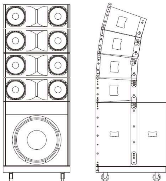
Floor Installation
