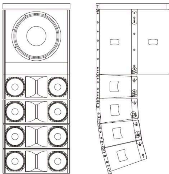
Hanging Installation
