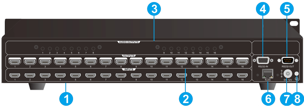
[Rear Panel]
