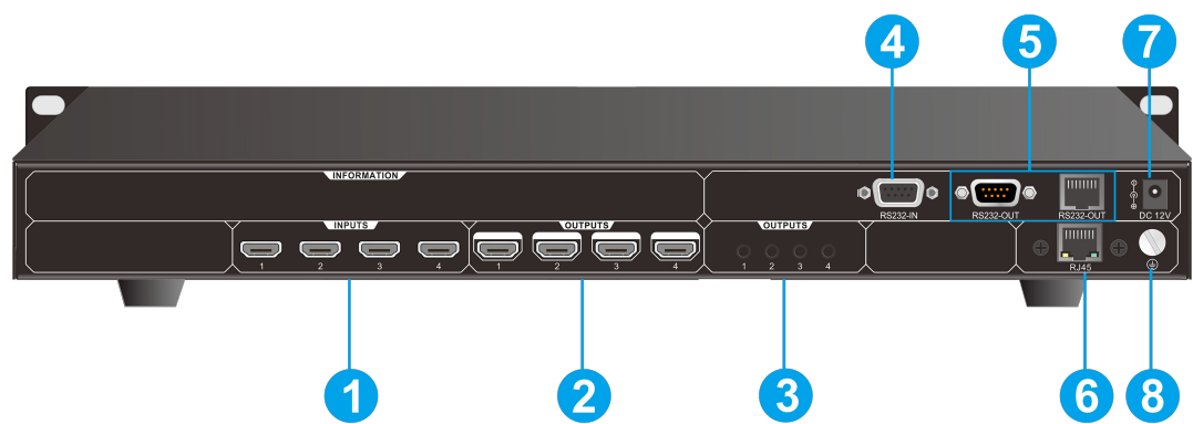
[Rear Panel]
