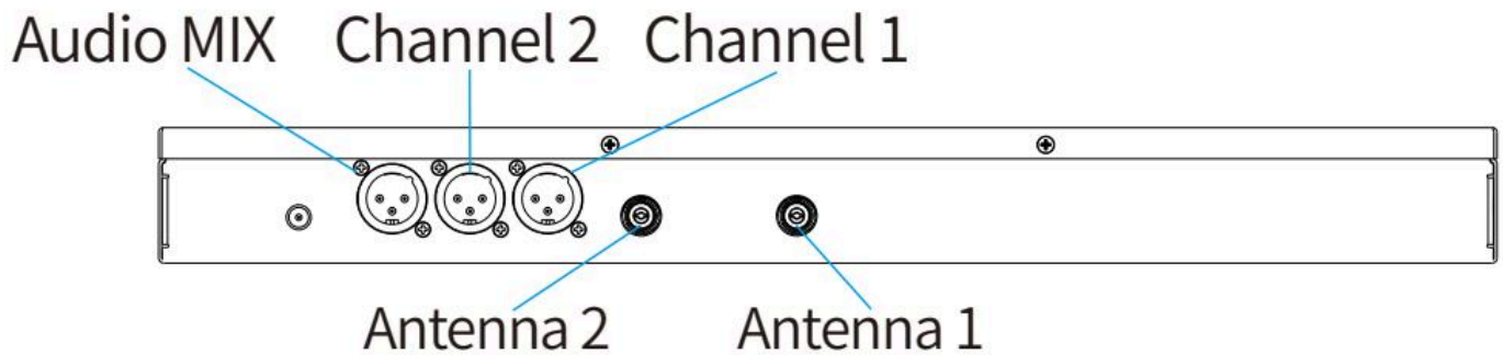
[ Rear Panel ]
